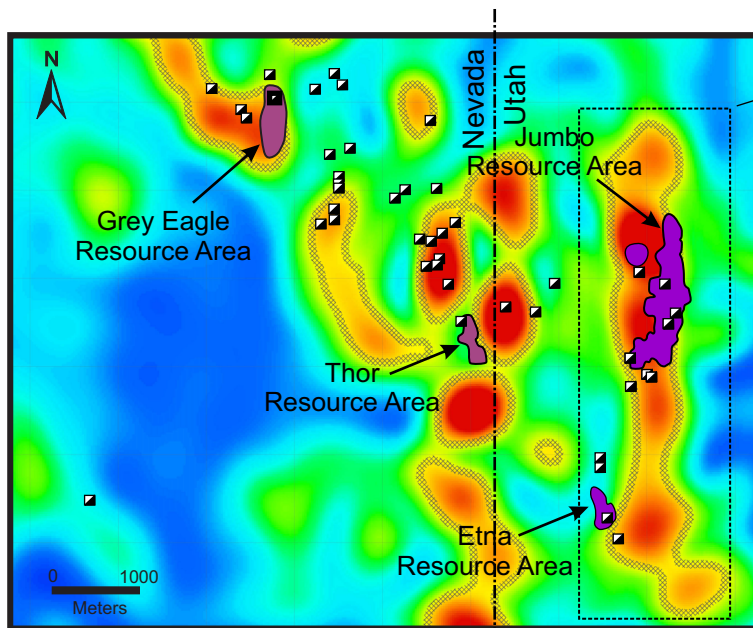
Gold Springs ZTEM anomaly at 375m below surface
